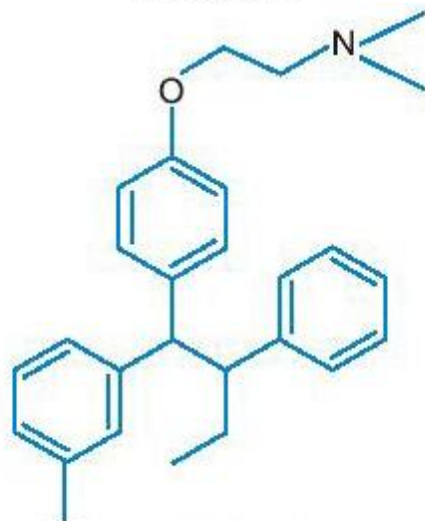
Droloxifene
