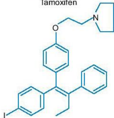
Idoxifene
