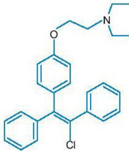
Clomiphene
