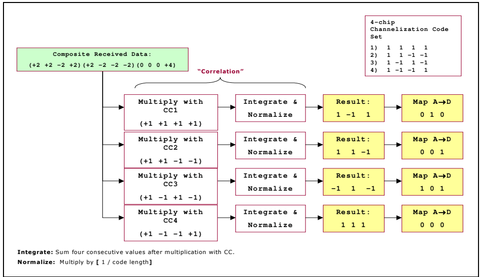
Figure 4.28: Channelization Coding example - Receiver.
